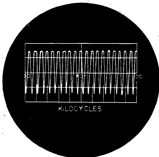
Clipped upper peaks indicating distorted sine wave.
