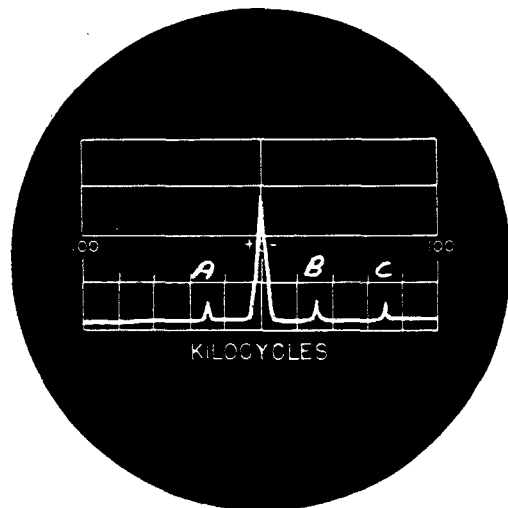
A and B—Sidebands due to 30KC supersonics. C—Parastic 70KC below Carrier.
