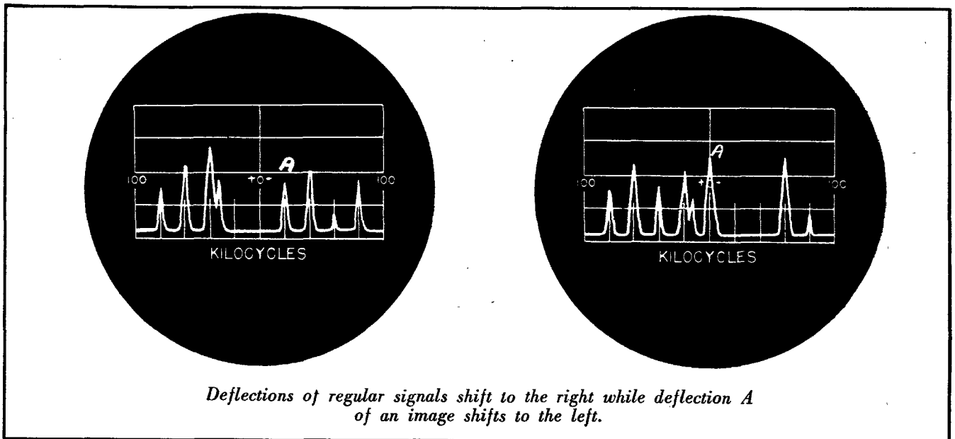
Figure 12. Direction of Travel of Images Against Regular Signals as Receiver is Tuned
